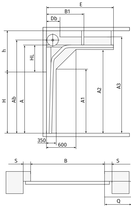
High lift with double bend
