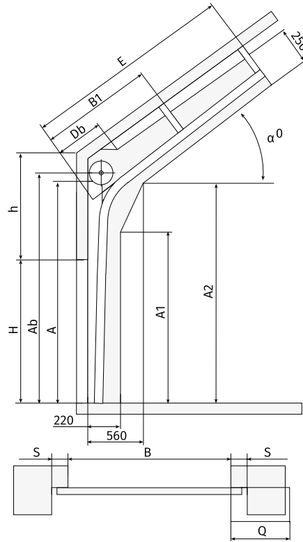
High inclined lift
