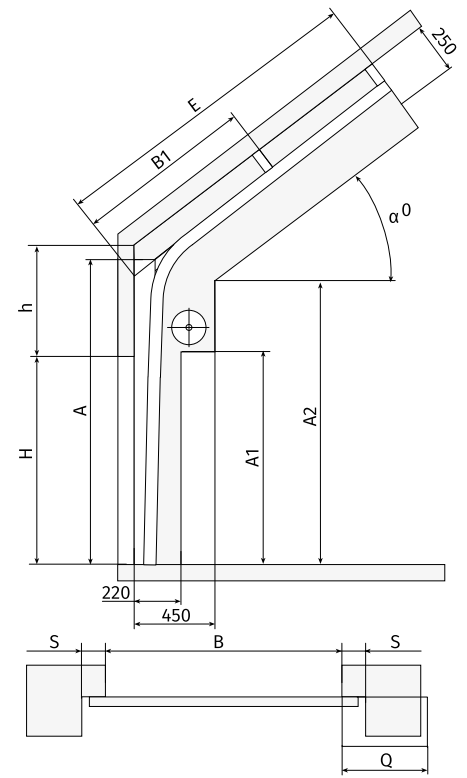
High inclined lift, low level cable drum
